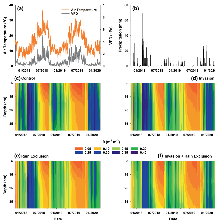
FIGURE 1 Air temperature and vapour pressure deficit (VPD) (a), precipitation (b) and volumetric water content ( \theta ) for Control (c), Invasion (d), Rain Exclusion (e) and Invasion + Rain Exclusion (f) within the soil profile. \theta was measured in 0.05, 0.20 and 0.40 m depth ( n = 6 per treatment and depth), which is in the range of the rooting depths for both investigated species. In plots (c–e), \theta (colour scale) is shown in a soil profile (y-axis) over time (x-axis). Red and orange colours indicate low water availability, green colours depict medium water availability and bluish colours show high water availability.
