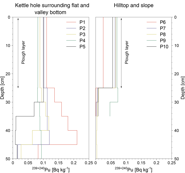
Figure 3. Depth distribution of ^{239+240}\text{Pu} at different geomorphological positions. Locations P1 to P10 are given in Fig. 1.
