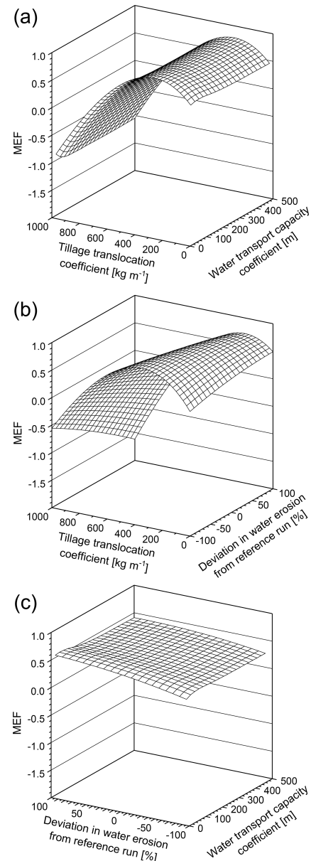
Figure 6. Inverse modelling of tillage and water erosion compared to ^{239+240}\text{Pu} -derived soil redistribution. Three parameter combinations (tillage transport coefficient, k_{til} ; water transport capacity coefficient, k_{tc} ; deviation in water erosion strength compared to reference parameterisation) are tested on their effect on the goodness-of-fit, represented by the MEF (model efficiency coefficient: perfect model fit = 1; model prediction as good as the mean = 0; model prediction worse than mean = < 0).
