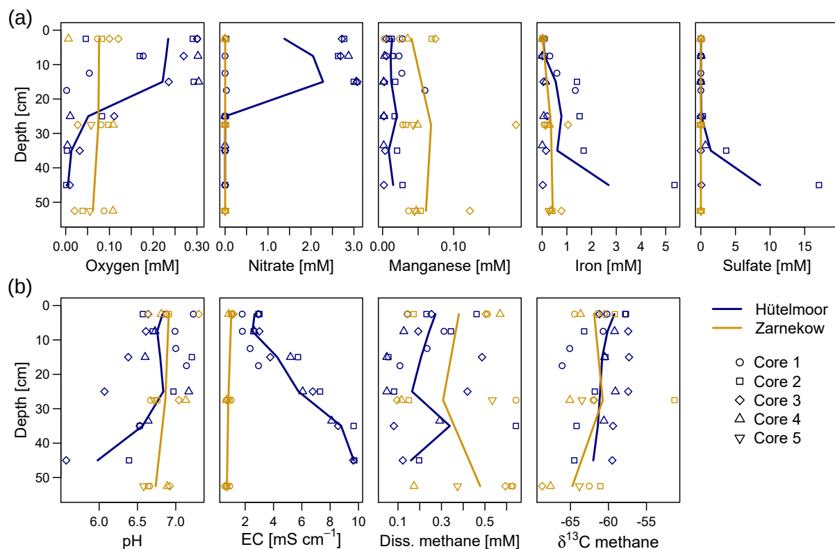
Figure 2. Depth profiles of oxygen, nitrate, total iron, manganese, and sulfate (a), and profiles of pH, EC, dissolved methane, and the isotopic signature of methane-bound carbon (b) in both study sites. Solid lines connect the respective means of individual wetlands ( n = 4 for Hütelmoor and n = 5 for Zarnekow).
