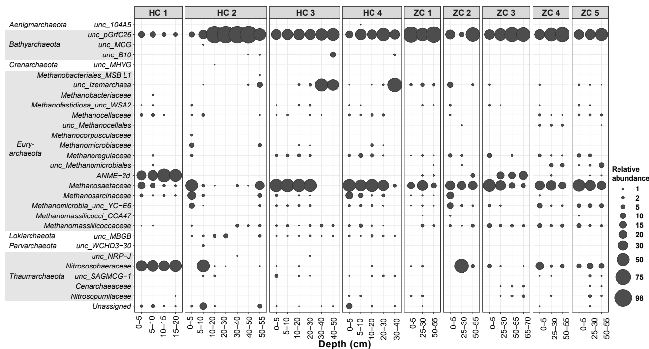
Figure 5. Relative abundances of different archaeal lineages in the study sites. Along the horizontal axis samples are arranged according to site and depth. The rank order along the vertical axis is shown for the family level. If an assignment to the family level was not possible, the next higher assignable taxonomic level was used.
