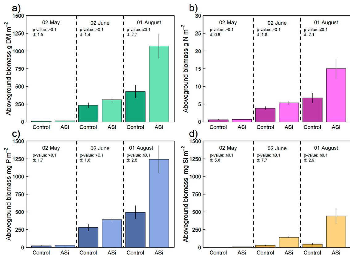
FIGURE 2 Results of the three biomass sampling campaigns (02/05/2024, 02/06/2024 and 01/08/2024) during the crop growth period 2023 with (A) barley biomass yield [g dry mass (DM) m -2 ] and nutrient uptake for (B) N (g N m -2 ), (C) P (mg P m -2 ) and (D) silica (Si; mg Si m -2 ). Error bars indicate \pm SE.
