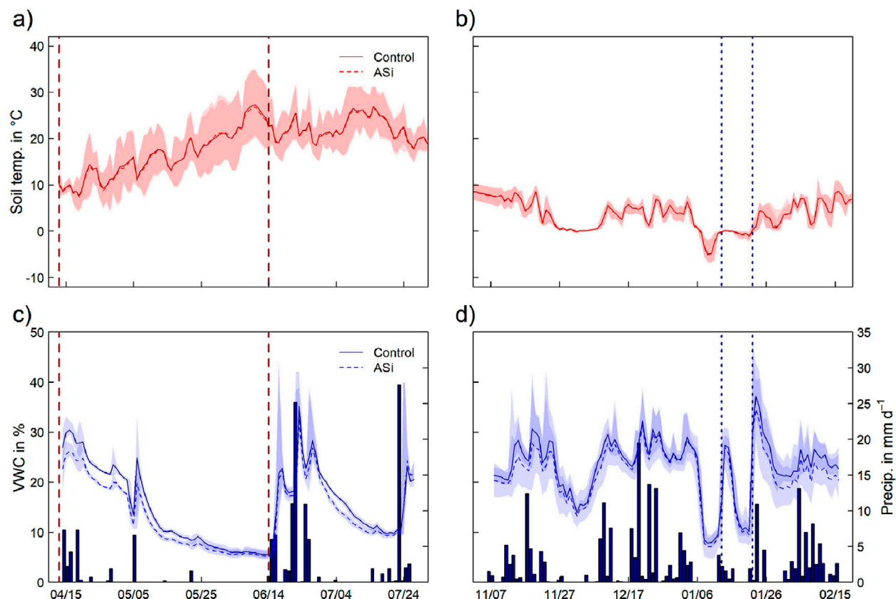
FIGURE 1 Course of soil temperature (°C; solid red line for C and dashed red line for Si) at 6 cm soil depth (A,B), soil moisture (volumetric water content (VWC) in %; solid blue line for C and dashed blue line for Si) and precipitation (mm d -1 ) (C,D) for the crop growth and following fallow period in 2023 (A,C) and 2023/2024 (B,D) at the study site in Müncheberg. Dashed red vertical lines indicate the two fertilization events. Dotted blue lines represent soil thawing. Shaded areas represent the daily magnitude of measured soil temperature and soil moisture.
