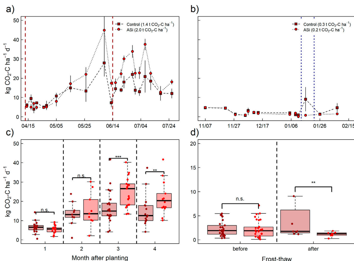
FIGURE 4 Results of periodically measured CO 2 emissions (kg CO 2 -C ha -1 d -1 ) for C (light red dots) and Si (dark red dots) during the (A) crop growth and (B) following fallow period in 2023 and 2023/2024, respectively. Error bars indicate \pm SE. (Figures 3C, D) shows boxplots of CO 2 emissions grouped by period after planting (summer period) and before (C) vs. after frost-thaw (D) (winter period). Significant differences (Wilcoxon-test) between the Treatments within each group are indicated by asterisks (p-value: *** < 0.01, ** < 0.05, * < 0.1, n.s. > 0.1).
