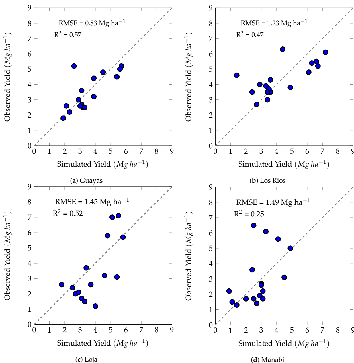
Figure 6. Observed vs. Simulated Yields ( \text{Mg ha}^{-1} ) from 2002 to 2018 in (a) Guayas, (b) Los Rios, (c) Loja and, (d) Manabi.
