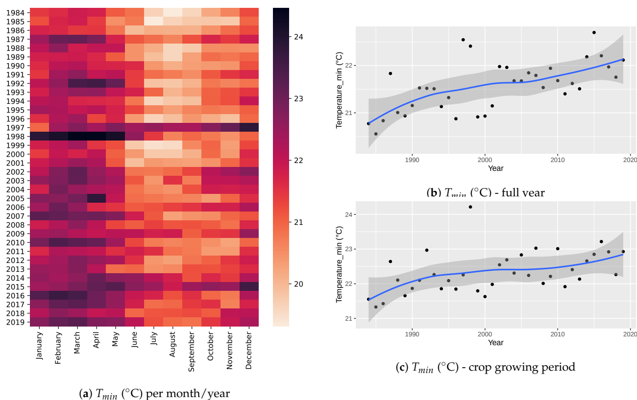
Figure 5. Time series of average minimum temperature (°C) in Manabi from 1984 to 2019. (a) Heat-map of T_{min} (°C) per each month and year. The color scale represents the temperature in °C. (b) T_{min} (°C) averaged during the full year. (c) T_{min} (°C) averaged during the maize crop growing period in Ecuador (January–May). Each dot represents one record, the blue line shows the smoothed time series and the shaded area represents the 95% confidence interval.
