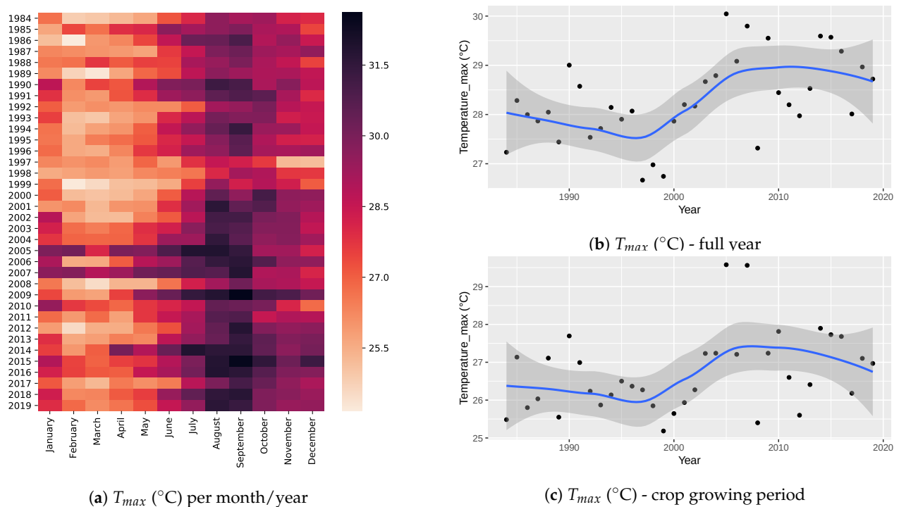
Figure 3. Time series of average maximum temperature (°C) in Los Rios from 1984 to 2019. (a) Heat-map of T_{max} (°C) per each month and year. The color scale represents the temperature in °C. (b) T_{max} (°C) averaged during the full year. (c) T_{max} (°C) averaged during the maize crop growing period in Ecuador (January–May). Each dot represents one record, the blue line shows the smoothed time series and the shaded area represents the 95% confidence interval.
