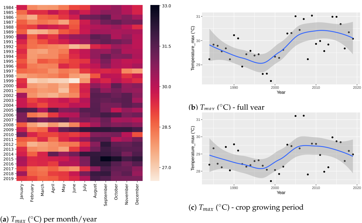
Figure A13. Time series of average maximum temperature (°C) in Manabi from 1984 to 2019. (a) Heat-map of T_{max} (°C) per each month and year. The color scale represents the temperature in °C. (b) T_{max} (°C) averaged during the full year. (c) T_{max} (°C) averaged during the maize crop growing period in Ecuador (January–May). Each dot represents one record, the blue line shows the smoothed time series and the shaded area represents the 95% confidence interval.
