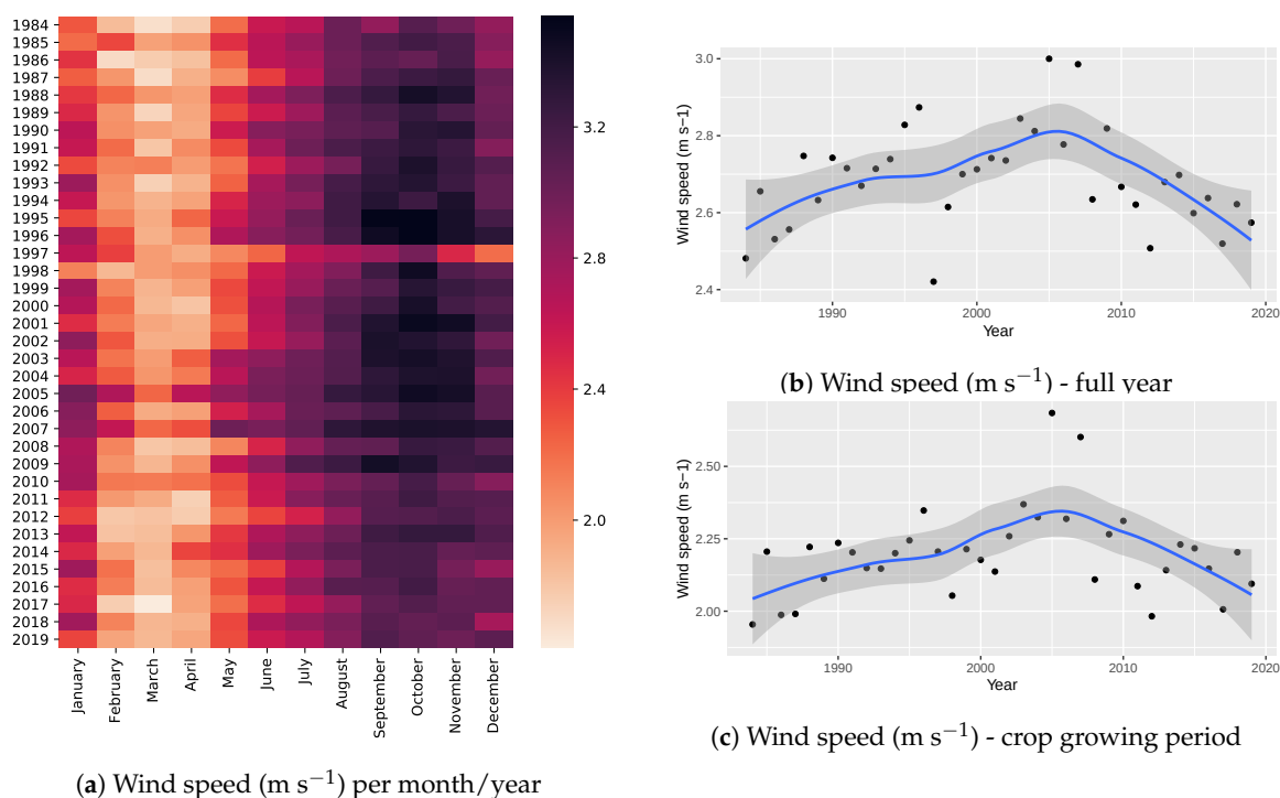
Figure A15. Time series of average wind speed ( \text{m s}^{-1} ) in Manabi from 1984 to 2019. (a) Heat-map of wind speed ( \text{m s}^{-1} ) per each month and year. The color scale represents the wind speed in \text{m s}^{-1} . (b) Wind speed averaged during the full year. (c) Wind speed averaged during the maize crop growing period in Ecuador (January–May). Each dot represents one record, the blue line shows the smoothed time series and the shaded area represents the 95% confidence interval.
