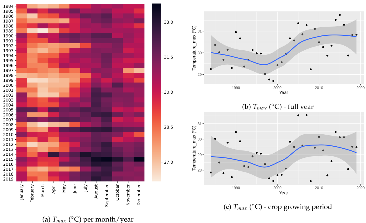
Figure A1. Time series of average maximum temperature (°C) in Guayas from 1984 to 2019. (a) Heat-map of T_{max} (°C) per each month and year. The color scale represents the temperature in °C. (b) T_{max} (°C) averaged during the full year. (c) T_{max} (°C) averaged during the maize crop growing period in Ecuador (January–May). Each dot represents one record, the blue line shows the smoothed time series and the shaded area represents the 95% confidence interval.
