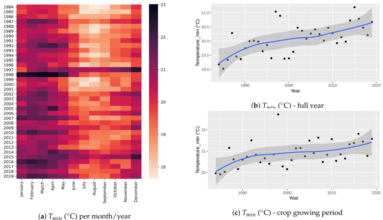
Figure 2. Time series of average minimum temperature (°C) in Guayas from 1984 to 2019. (a) Heat-map of T_{min} (°C) per each month and year. The color scale represents the temperature in °C. (b) T_{min} (°C) averaged during the full year. (c) T_{min} (°C) averaged during the maize crop growing period in Ecuador (January–May). Each dot represents one record, the blue line shows the smoothed time series and the shaded area represents the 95% confidence interval.
