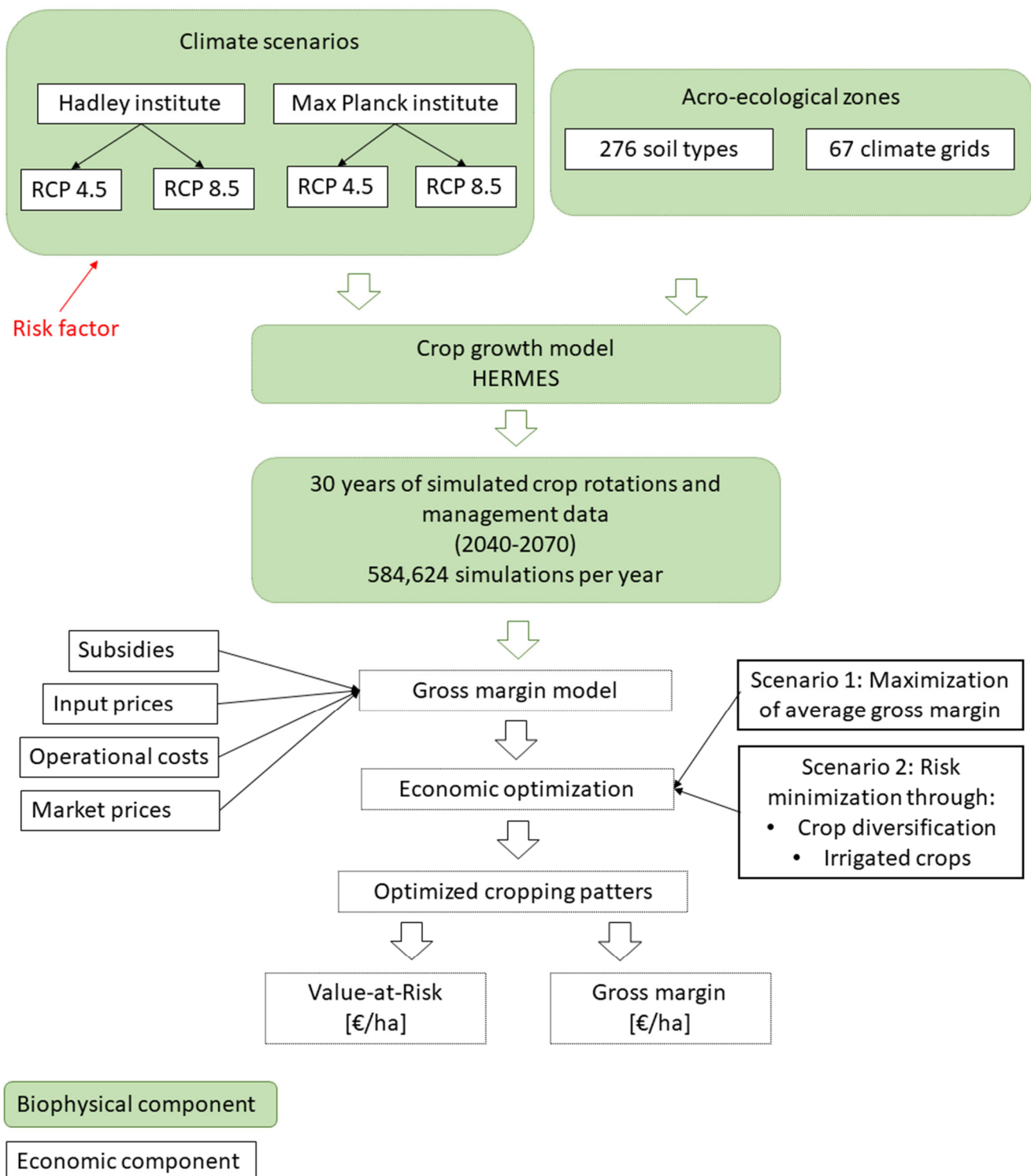
Figure 1. Model overview.
