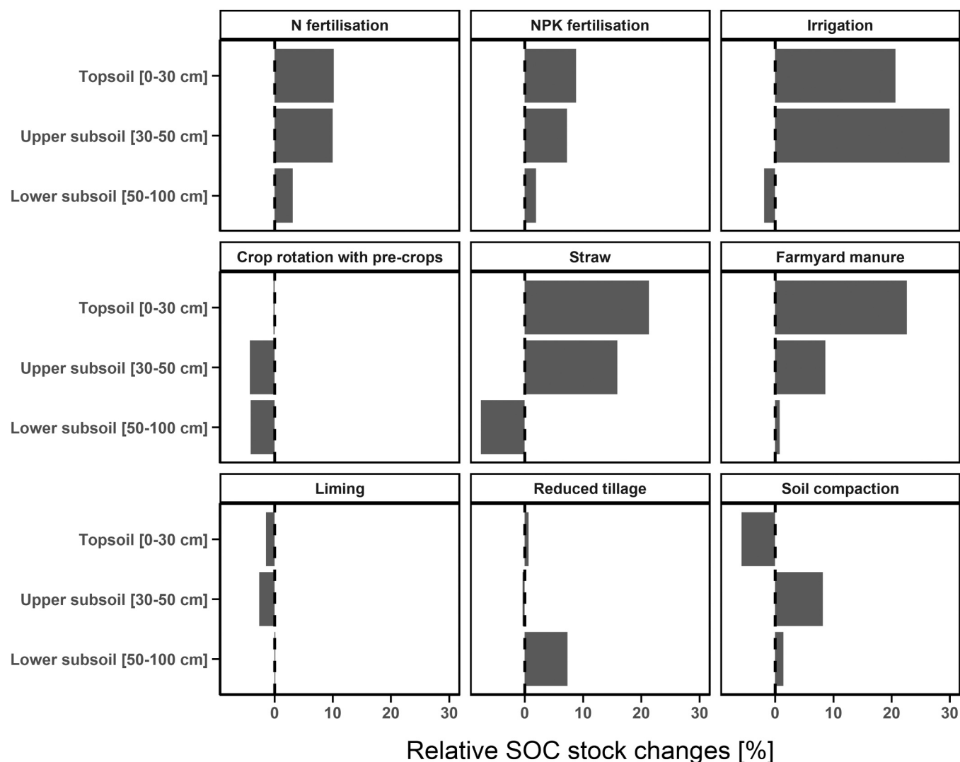
Fig. 4. Relative soil organic carbon (SOC) stock changes ( C_r ) due to agricultural management practices compared with the SOC stock of the corresponding reference per depth interval.
